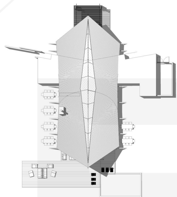
Main Facility Layout | Design Development
